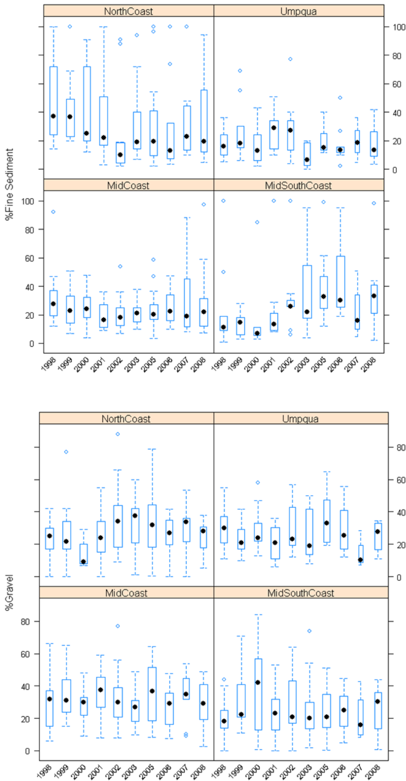
Figure 17. Boxplots of fine substrate and gravel in streams from 1998 – 2008.
