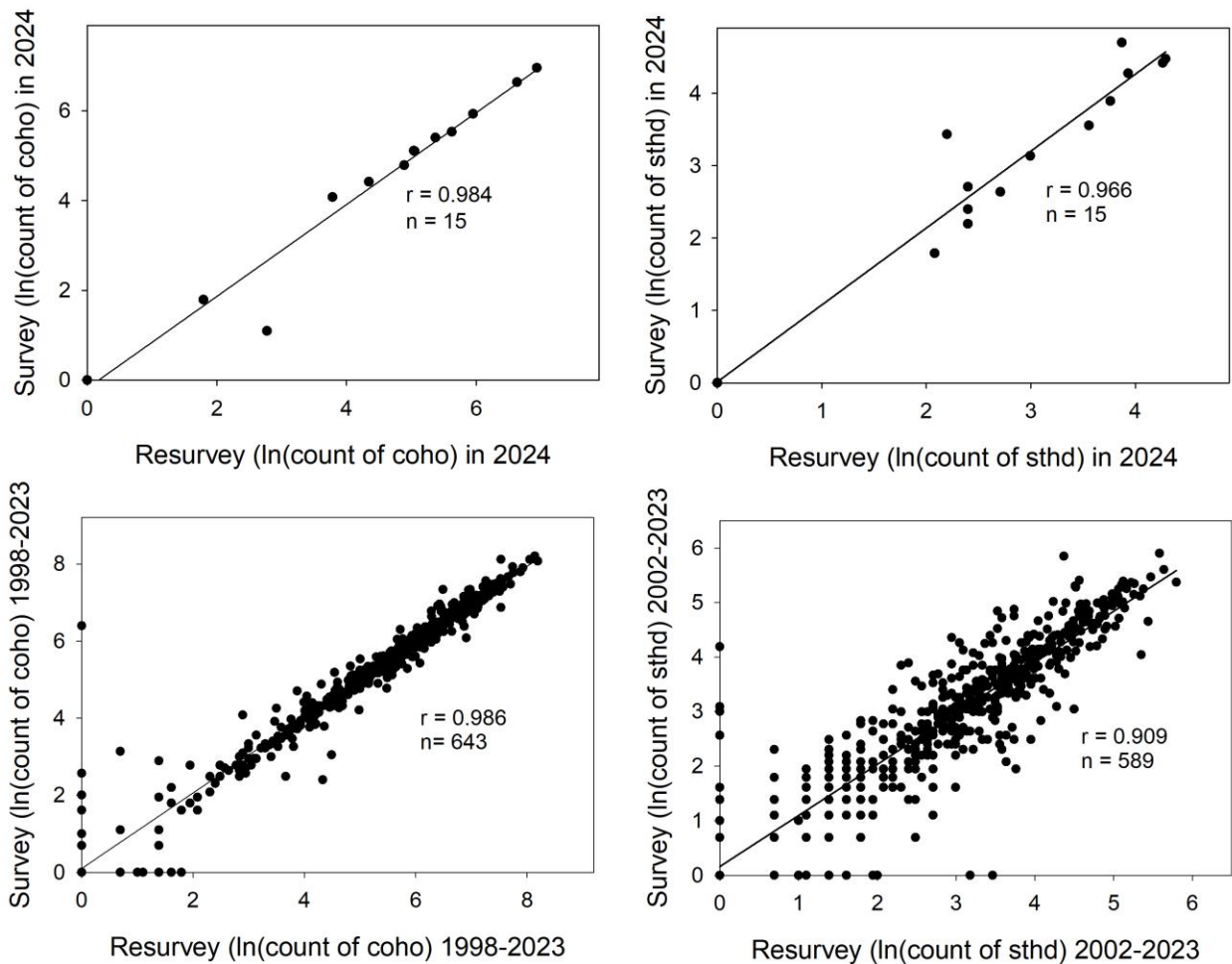
Figure 3. The relationship between Coho Salmon and steelhead parr counts from surveys and resurveys of the same sampling sites for 2024 (top panels) and for previous years (bottom panels). Data were log transformed to satisfy regression assumptions.
